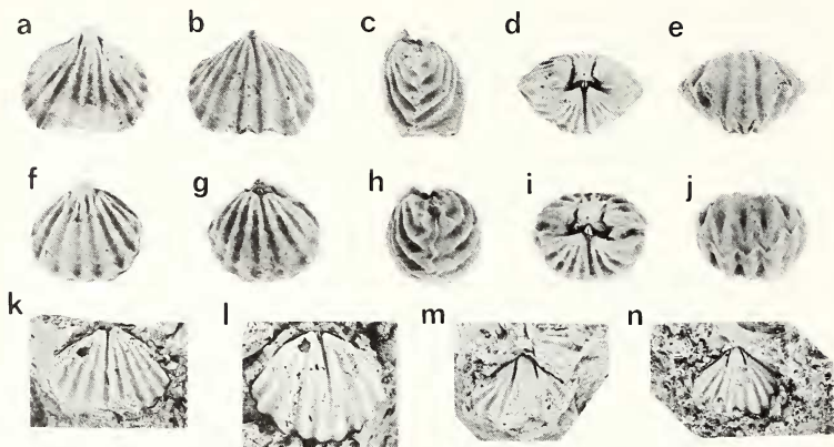
TEXT-FIG. 3. Topotype specimens of Stegerhynchus praecursor from the type locality, collected by Foerste, Clinton Bed, Clifton, Tennessee. Figs. a-e and f-j, pedicle, brachial, lateral, anterior, and posterior views of USNM 218094 and USNM 218098 respectively. Note cardinal process evident in figs. d and i. Fig. k, brachial valve of USNM 304184 showing extent of median elevation. Fig. l, brachial valve of USNM 218092 showing median elevation that is longer and more strongly developed than that in USNM 304184. Figs. m and n, pedicle valve of USNM 304185 and USNM 304186 showing dental lamellae.
